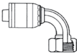
Female FOR-SEAL® (ORS) Short Drop Swivel, 90° Tube Elbow
