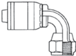
JIC/37° Female Swivel, 90° Elbow
