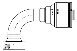
FLB - SAE Code 61 Flange 90° Elbow
