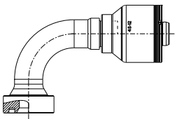
FHB - SAE Code 62 Flange 90° Elbow
