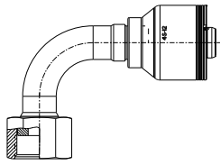
FRB - Female ORS Swivel 90° Elbow
