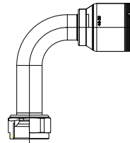
FJC - Female JIC/37° Swivel 90° Elbow - Long Drop
