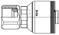
FJ - Female JIC/37° Swivel Straight
