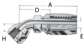
SAE 37° (JIC) swivel 45 elbow
