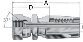
SAE 37° (JIC) swivel
