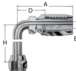
SAE 37° (JIC) swivel 90 elbow (short)
