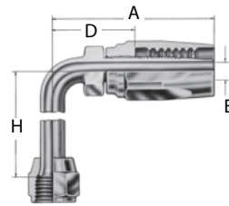
SAE 37° (JIC) swivel 90° elbow
